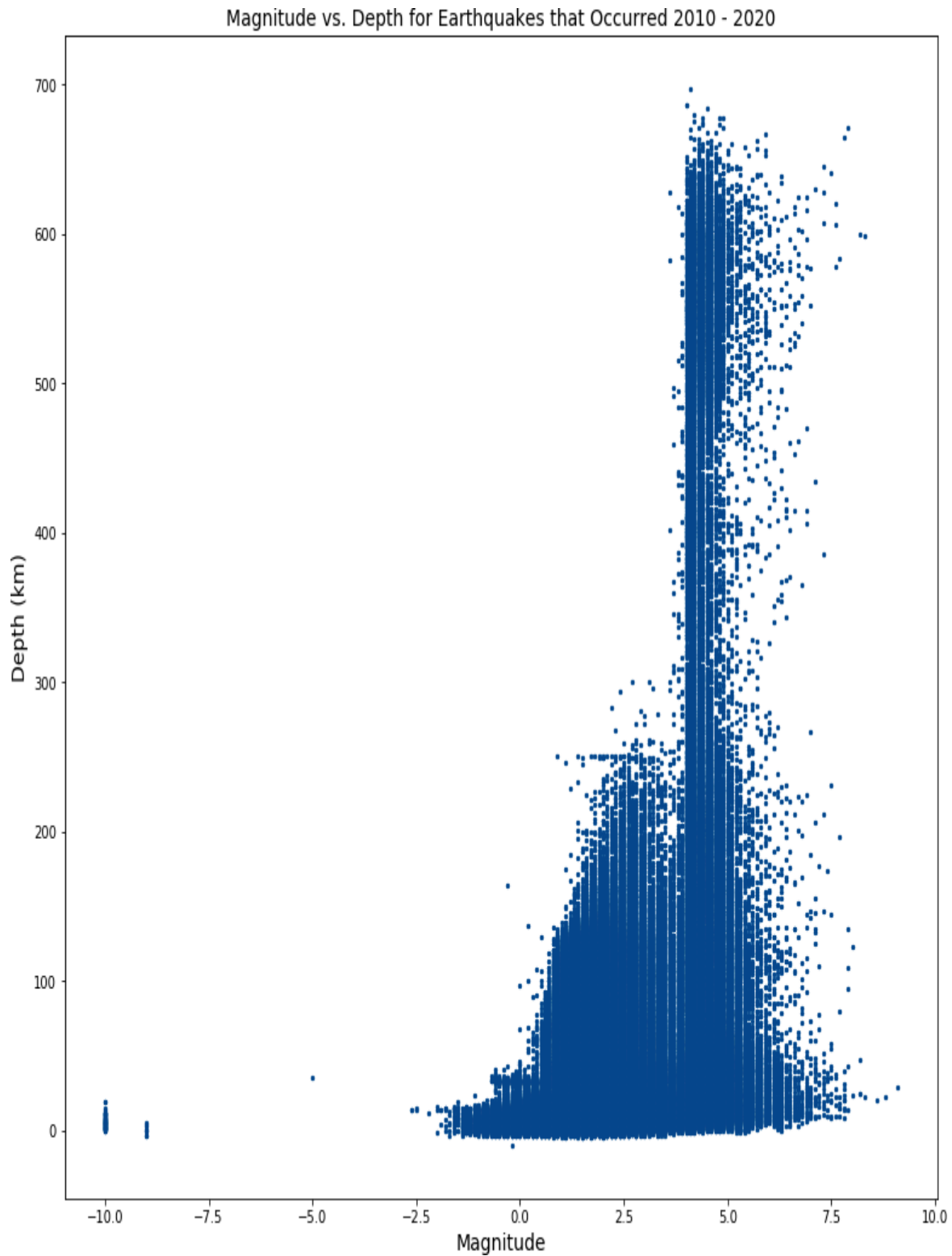
Figure 6-5. Scatter plot of the magnitude and depth of earthquakes
