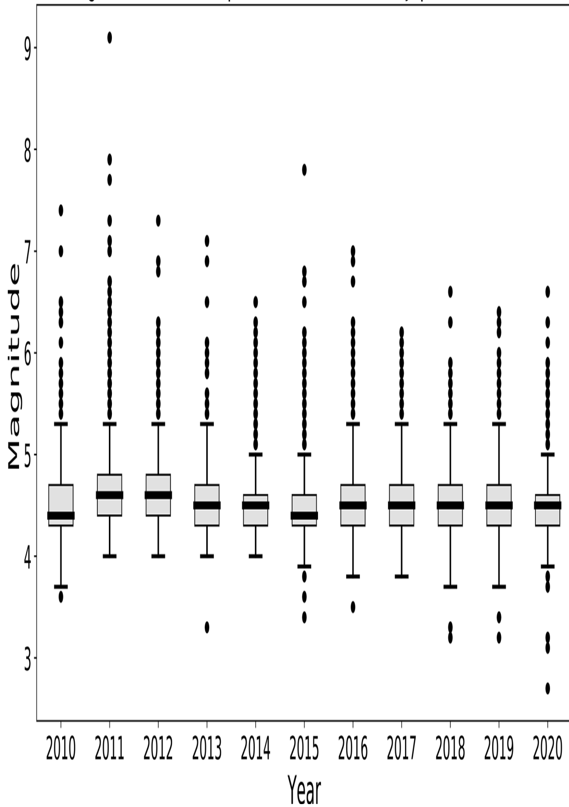
Magnitudes for Earthquakes that Occurred in Japan 2010 - 2020
