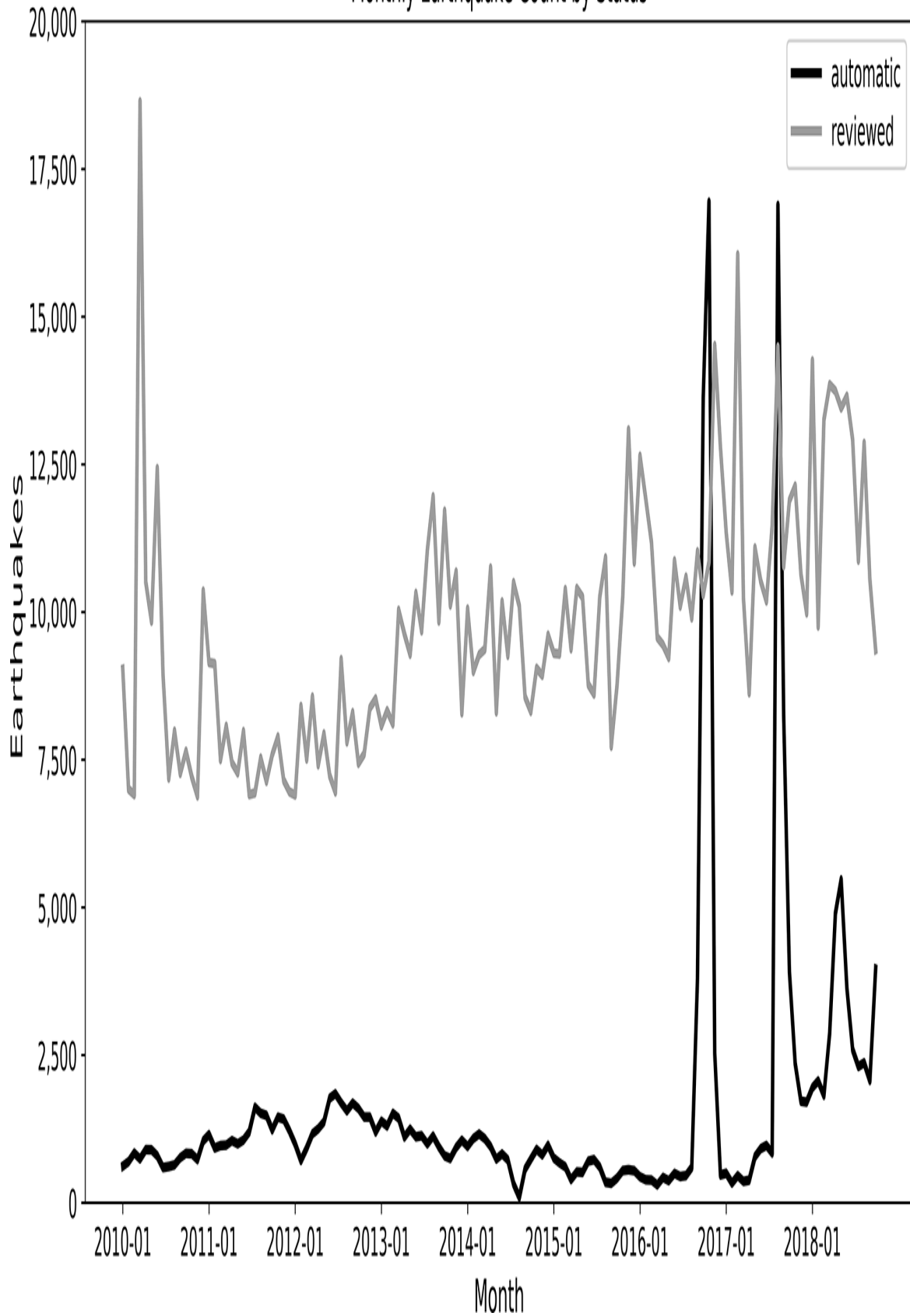
Monthly Earthquake Count by Status
