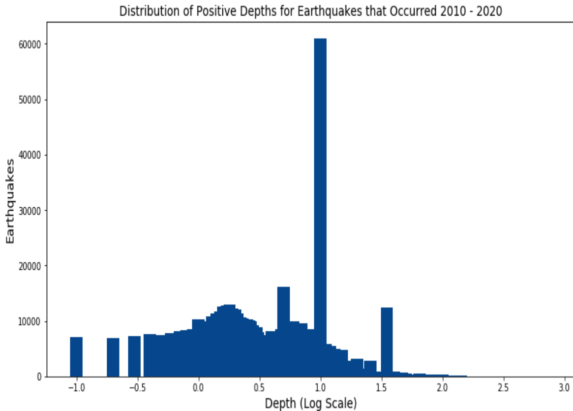
Figure 6-13. Distribution of earthquakes by depth on a log scale
