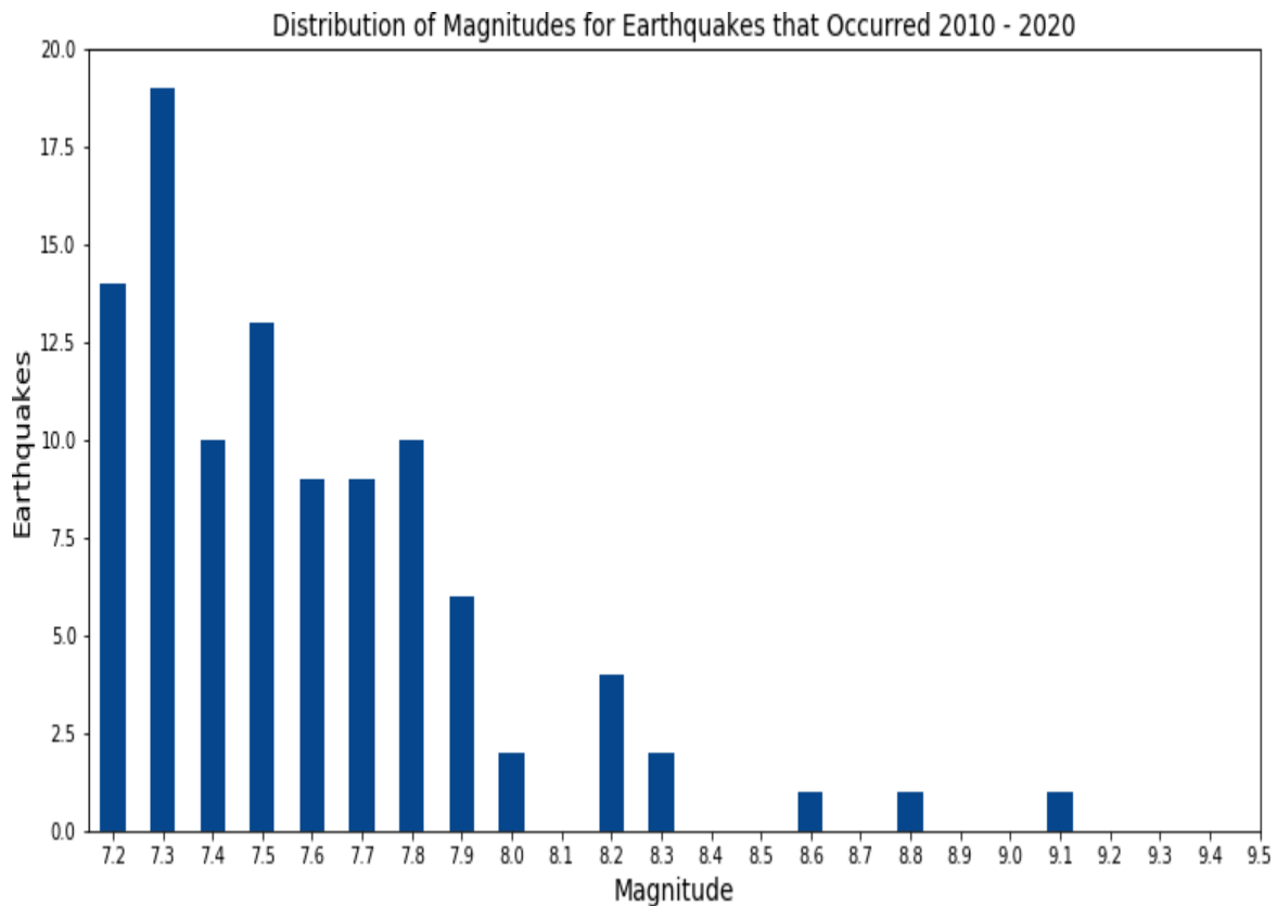
Figure 6-4. A zoomed-in view of the distribution of earthquake magnitudes, focused on the highest magnitudes
