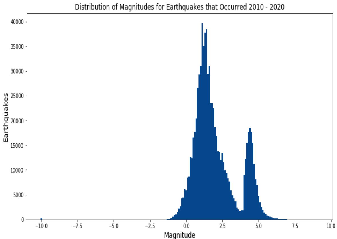
Figure 6-3. Distribution of earthquake magnitudes
