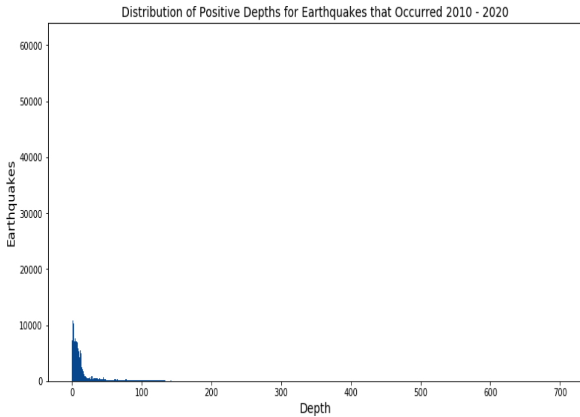
Figure 6-12. Distribution of earthquakes by depth, with unadjusted depths
