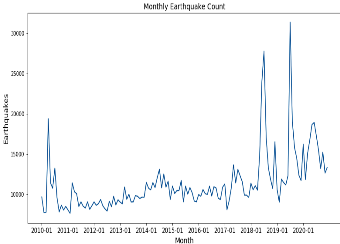
Figure 6-10. Number of earthquakes per month
