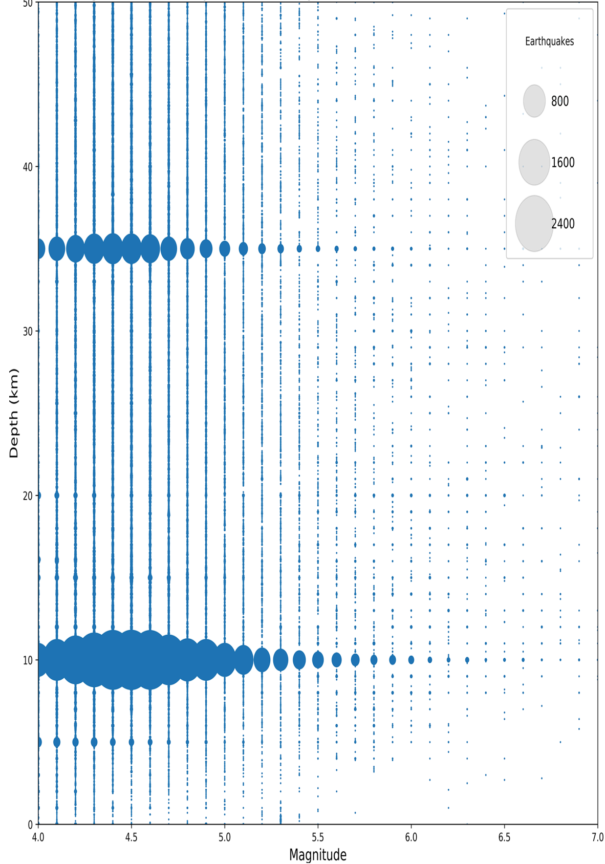
Magnitude vs. Depth for Earthquakes that Occurred 2010 - 2020
